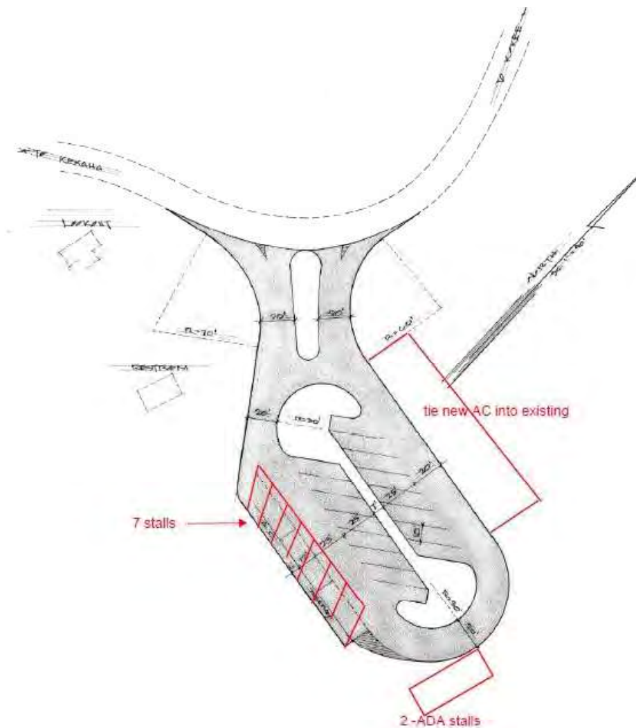
PUU HINAHINA LOOKOUT PARKING AREA SCALE: 1" = 40' *not to scale
